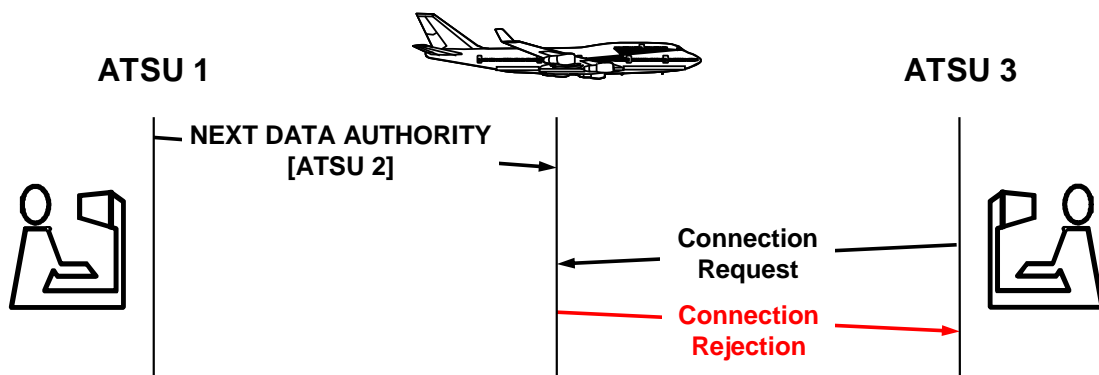
Figure 1-23. Connection request from an ATS unit not designated as the NDA
