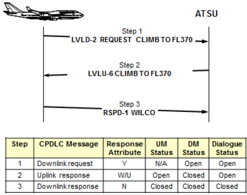
Figure 1-27. Message/dialogue status for CPDLC request and clearance exchange
